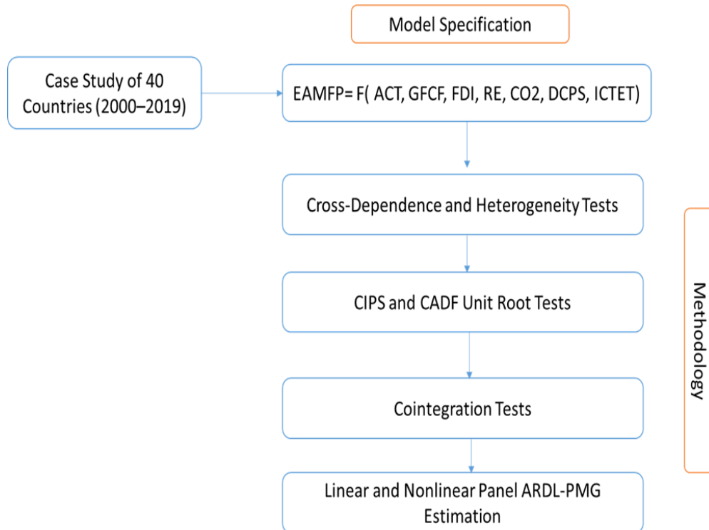
Figure 1. Methodology Framework.
